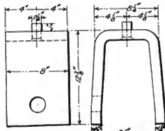
Figs. 1743-1744. Driving Box Saddle for Consolidation (2-8-0) Locomotive. American Locomotive Co.
